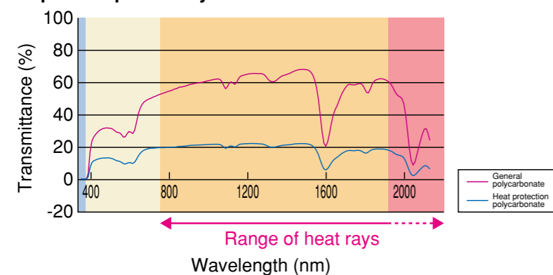
Graph1: Dispersed ray transmittance curve
